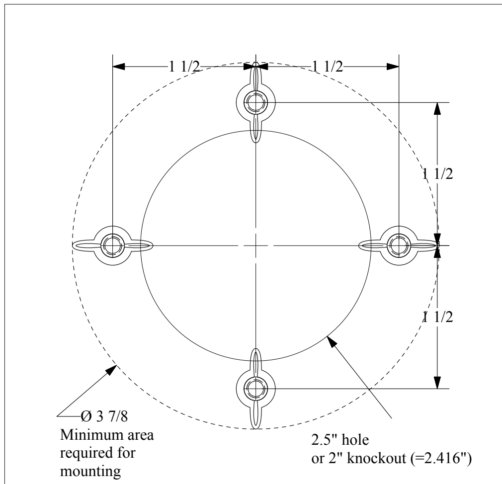
Mounting Template Scale 1:1
