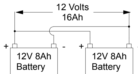
Batteries in Parallel
