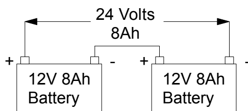
Batteries in Series
