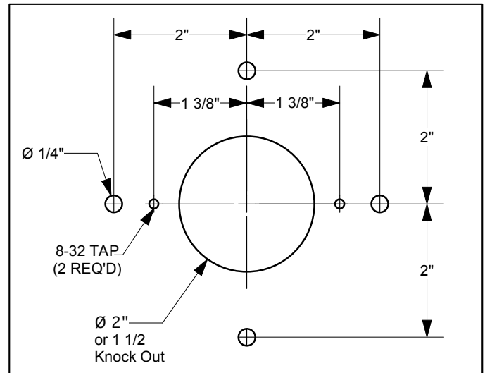
Hole Pattern For Mounting
