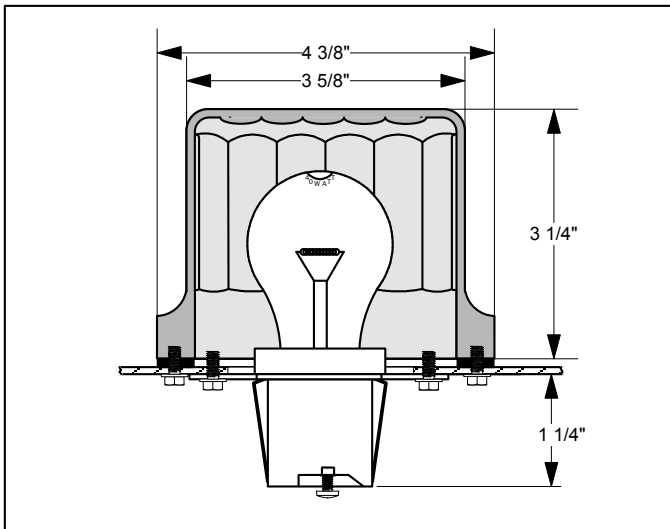
Cut-Away View
