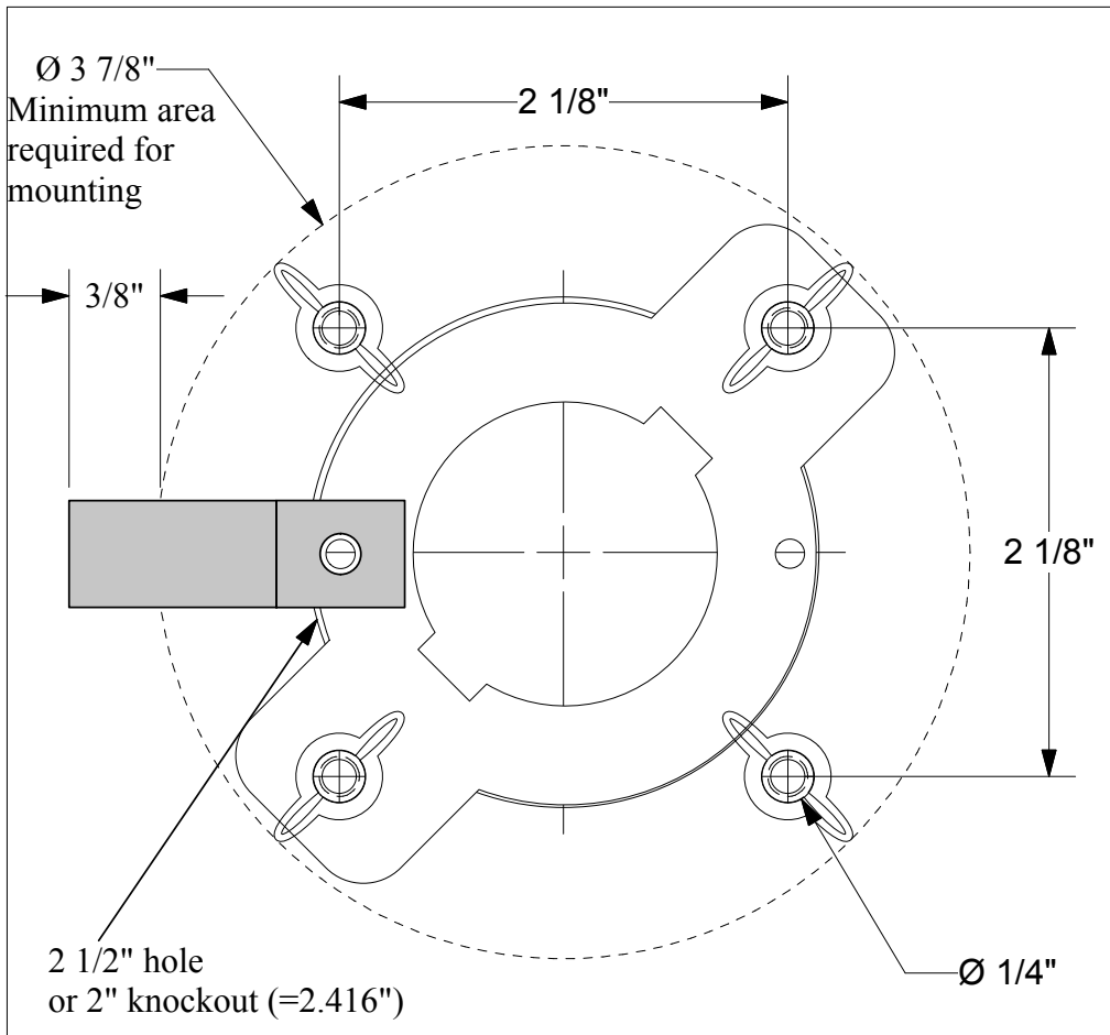
Mounting Templates
