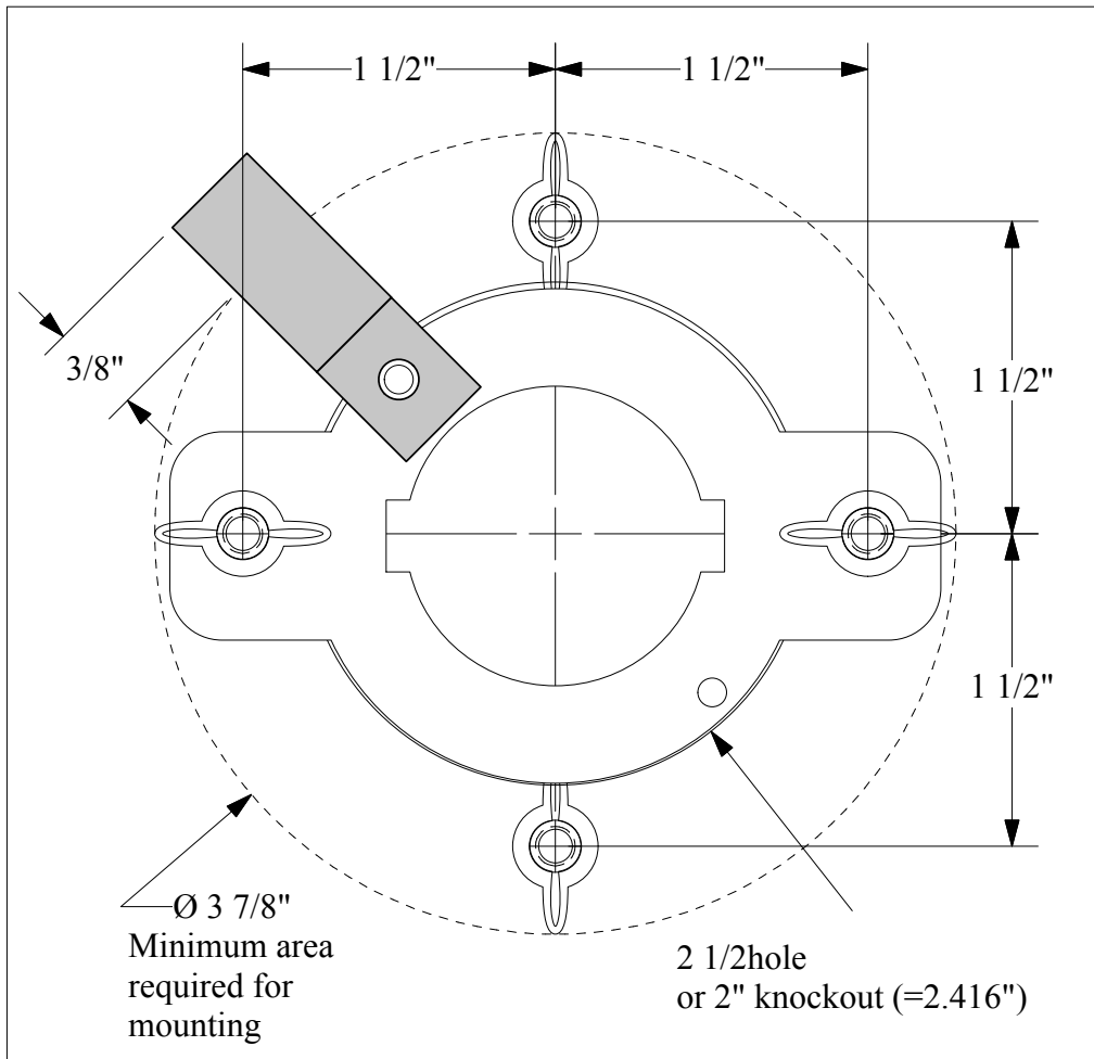
Mounting Templates
